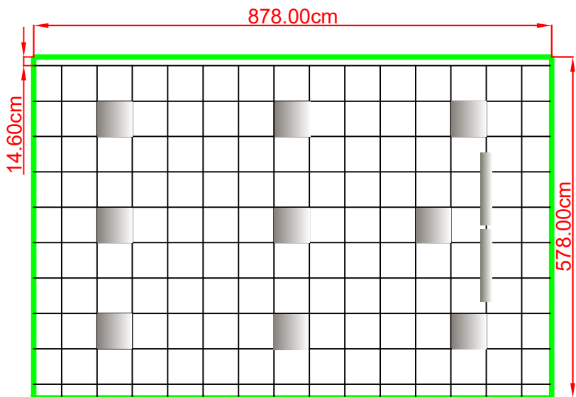
sala 61 h=3,18-3,20m
