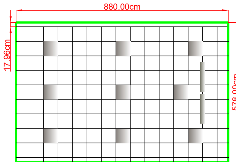
sala 62 h=3,18-3,19m
