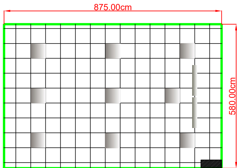
sala 43 h=3,18-3,20m
